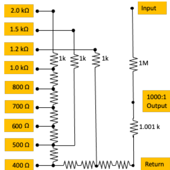
Figure 3. Voltage divider and load resistors. Unlabeled resistors are 100 Ω.
