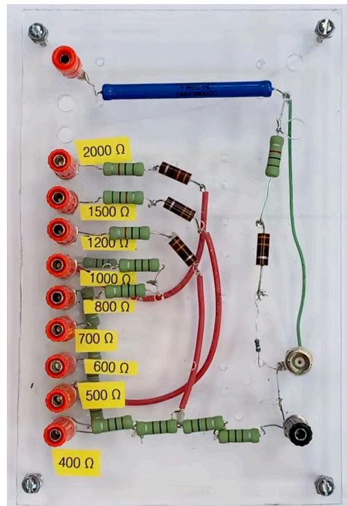
Figure 4. Voltage divider and load resistors.
